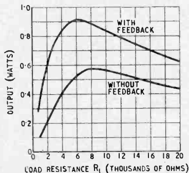
Fig. 6—Similar to Fig. 5, but using a small pentode.
