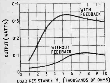
Fig. 5.—Results of an experiment on a small output triode, showing how the output—limited to 5 per cent. harmonic distortion—varies with load resistance.
