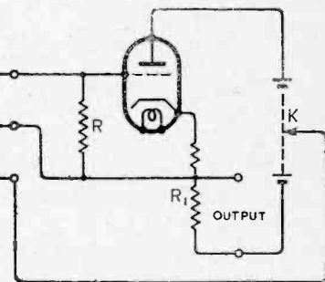
Neutralising surface leakage in piezo-crystal microphones.
