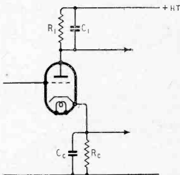
Fig. 3. The push-pull phase splitter is only a modified cathode follower and the analysis in the text applies to both if R_c = R_1 and C_c = C_1 .
