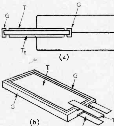
Neutralising surface leakage in piezo-crystal microphones.
