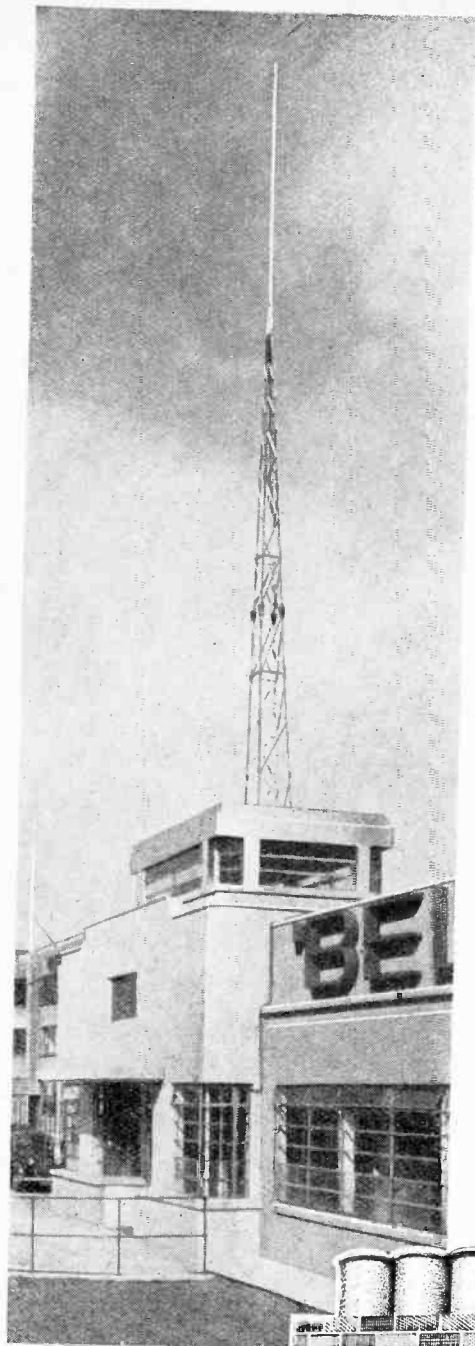
The illustration above shows the Belling-Lee Skytower Aerial—a 35 ft. lattice mast surmounted by an 18 ft. Skyrod.
